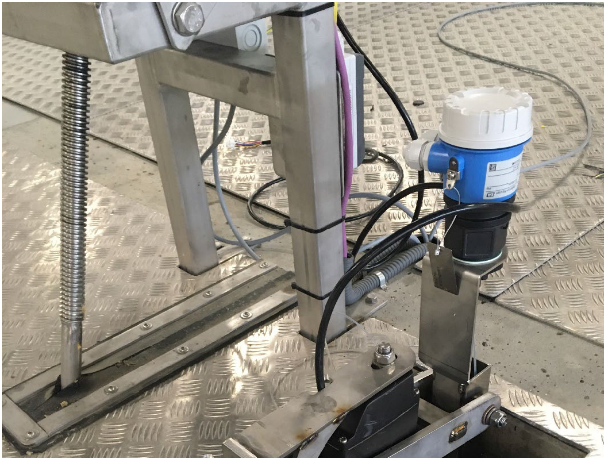
VE-Designed flow meter on inlet to process tanks.
